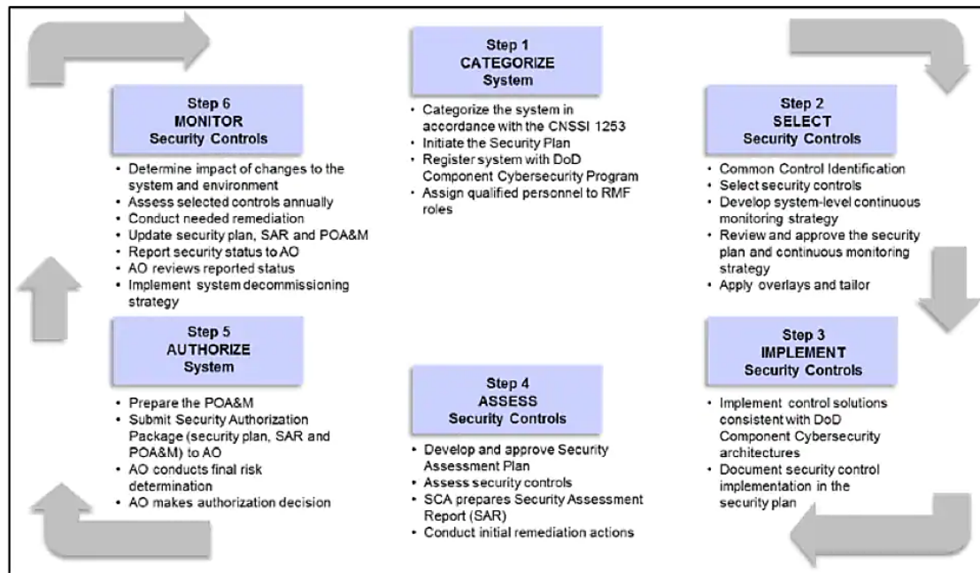
FIGURE 9 RMF PROCESS 38
